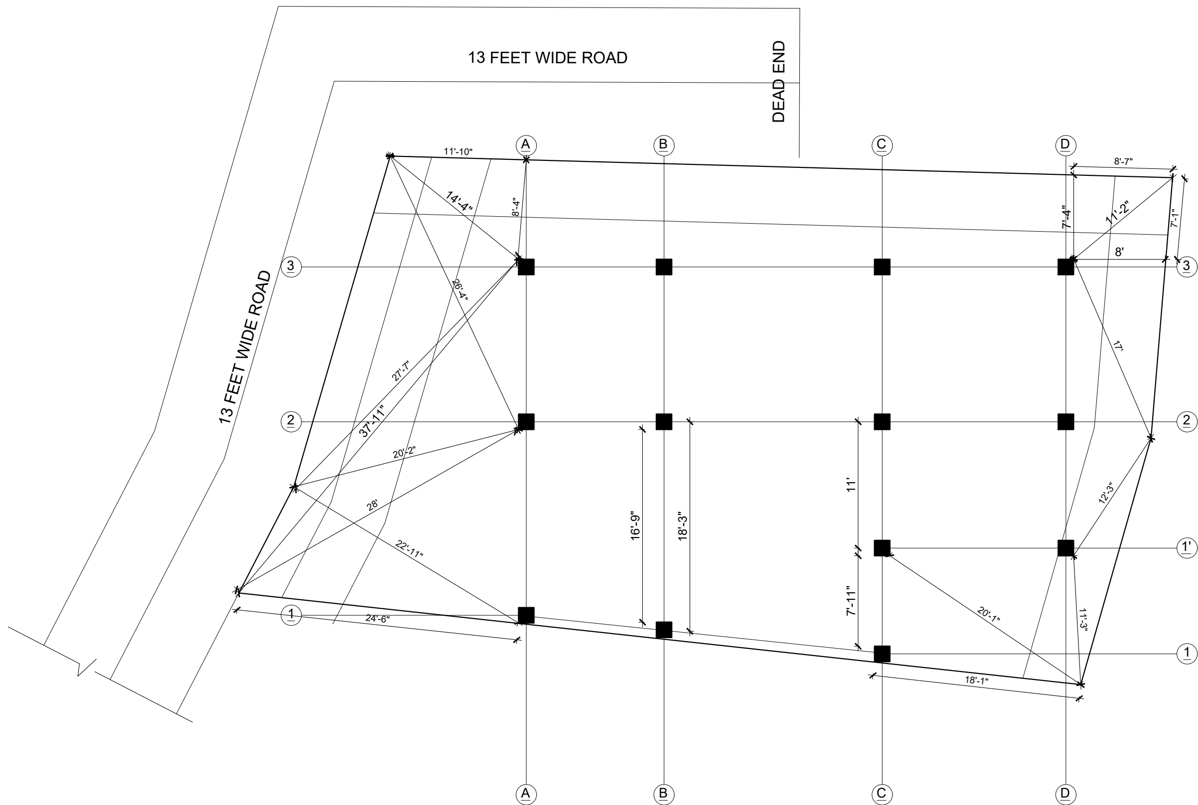
BASEMENT FLOOR PLAN FLOOR AREA: 1494 SQ.FT
