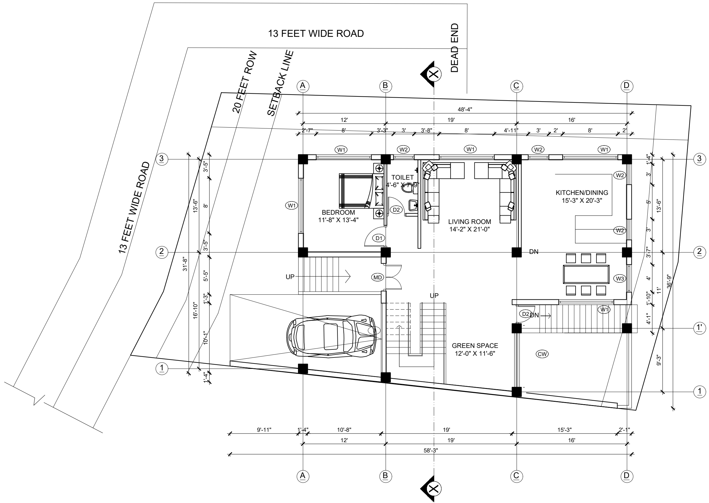
GROUND FLOOR PLAN FLOOR AREA: 1494 SQ.FT
