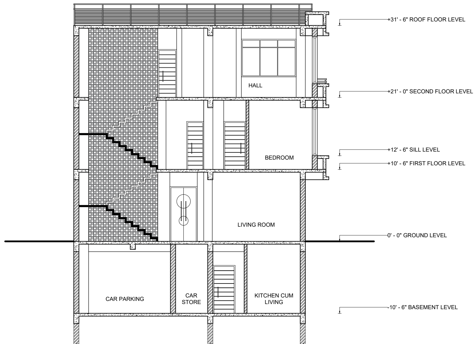
SECTION AT X-X
