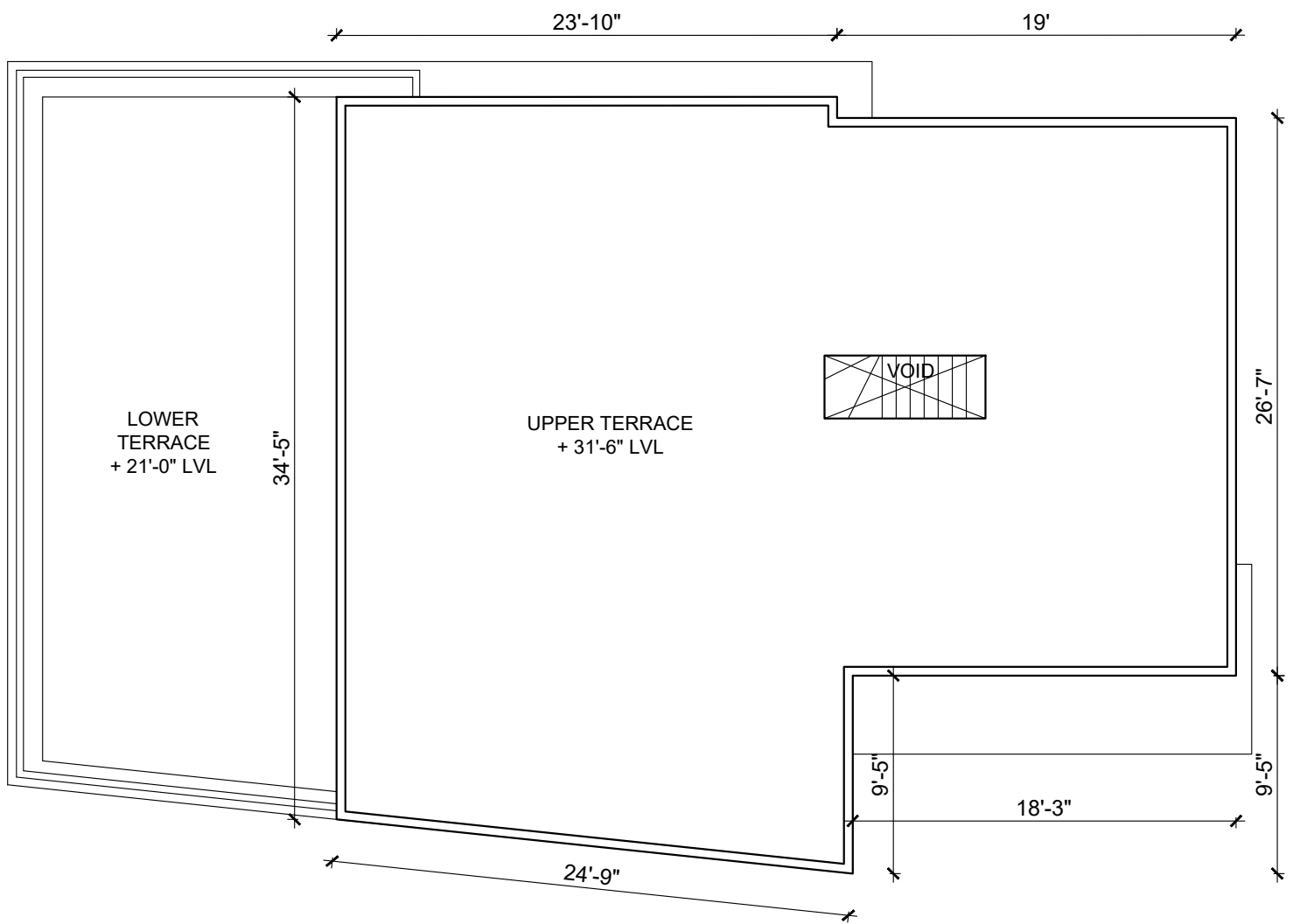
ROOF PLAN
