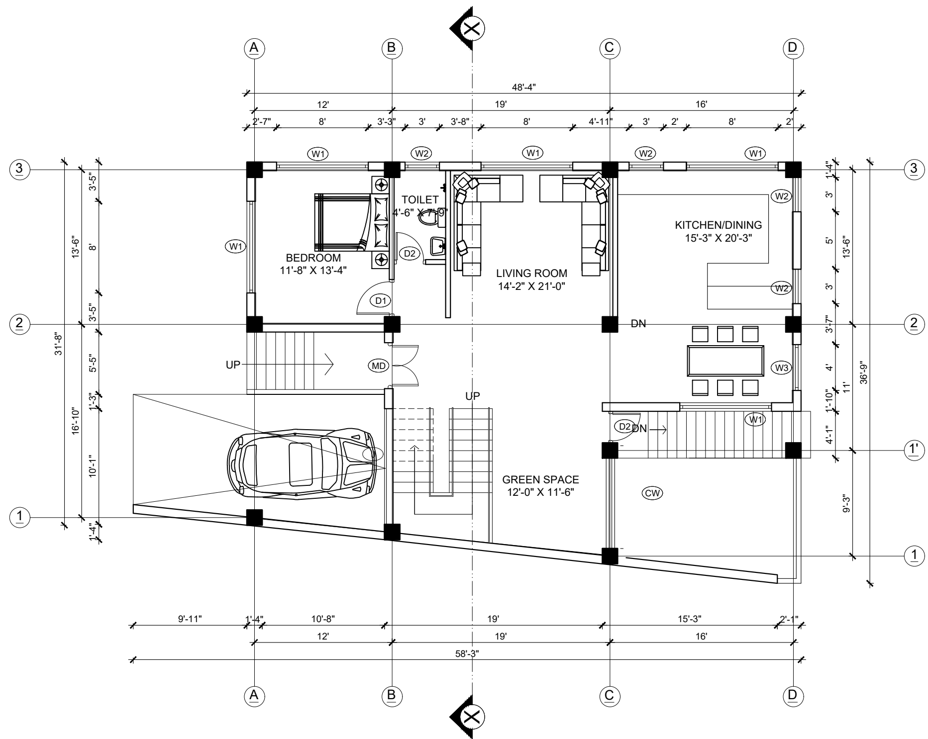
GROUND FLOOR PLAN FLOOR AREA: 1494 SQ.FT
