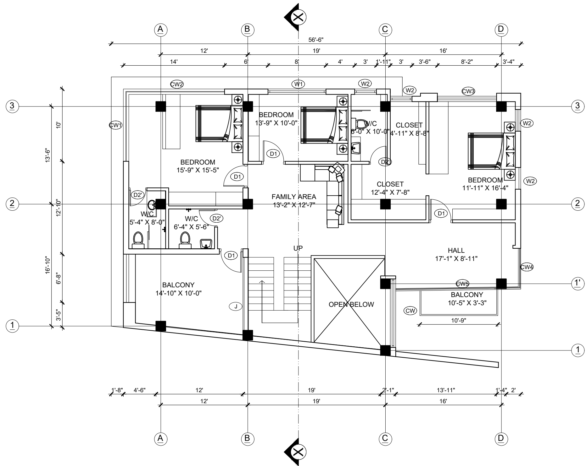
FIRST FLOOR PLAN FLOOR AREA: 1779 SQ.FT
